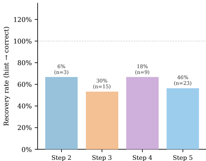
(B) Recovery Rate per Assembly Step (% = share of all filter activations at that step)
