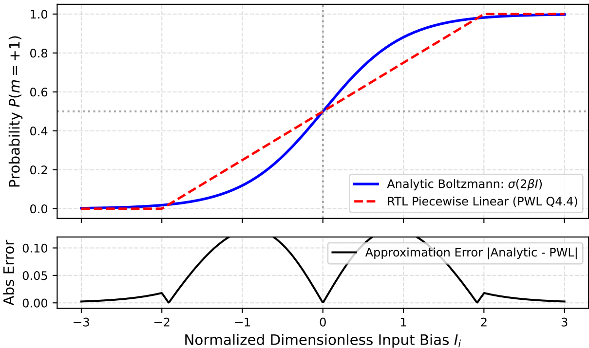
Fig. 1: Thermodynamic p-Bit Transfer Function ( \beta = 1.0 )
