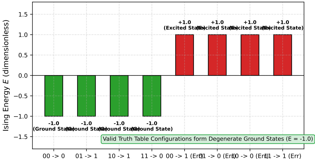
Fig. 2: Energy Landscape of Coupled XOR p-Bit Network with Hidden Unit H
