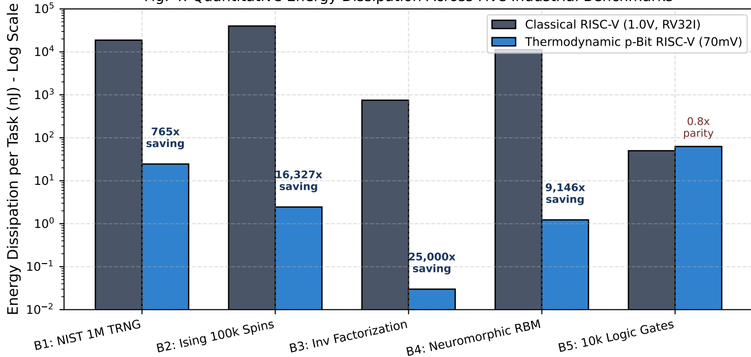
Fig. 4: Quantitative Energy Dissipation Across Five Industrial Benchmarks
