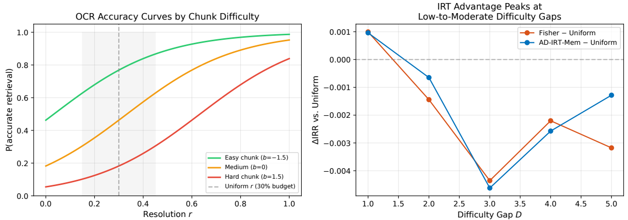
Figure 1: Left: OCR accuracy curves by chunk difficulty. For candidates in the concave (upper) region, marginal returns are similar, favoring uniform allocation. Right: \Delta IRR vs. uniform peaks at low difficulty gaps where some candidates span the convex region.
