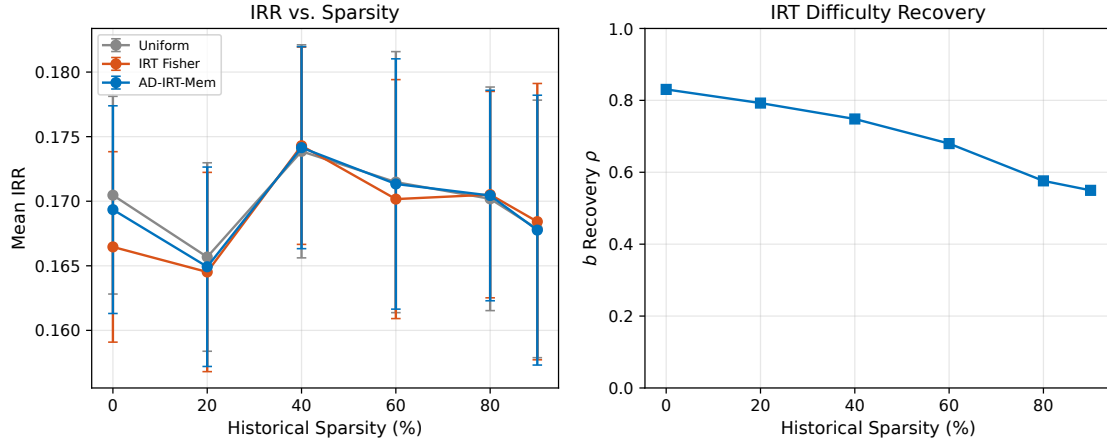
Figure 2: Left: IRR remains broadly similar across methods and sparsity levels. Right: IRT difficulty recovery \rho degrades with sparsity, as expected.
