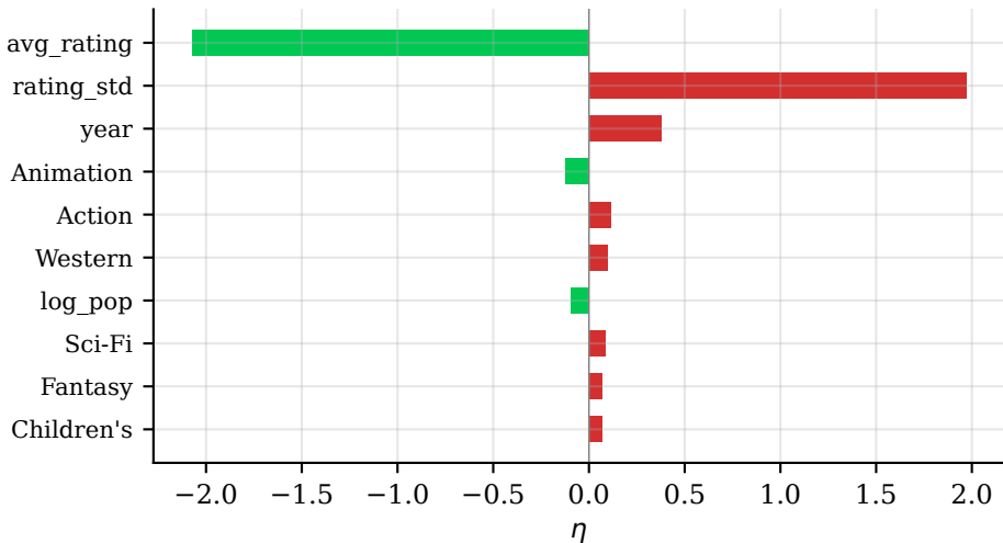
LLTM Weights (warm items, in-sample, seed 42)
