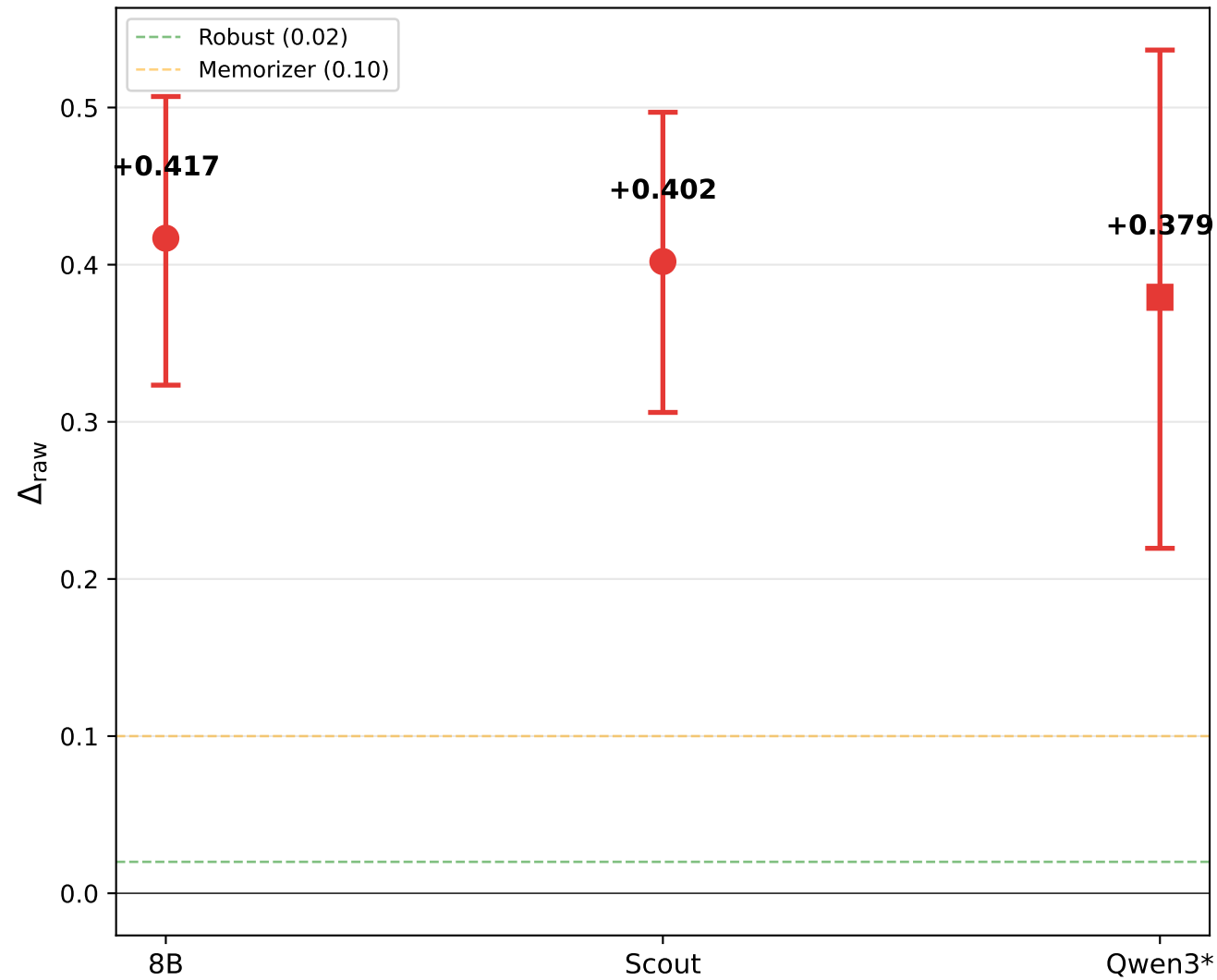
(A) Contamination Delta with 95% Bootstrap CI
