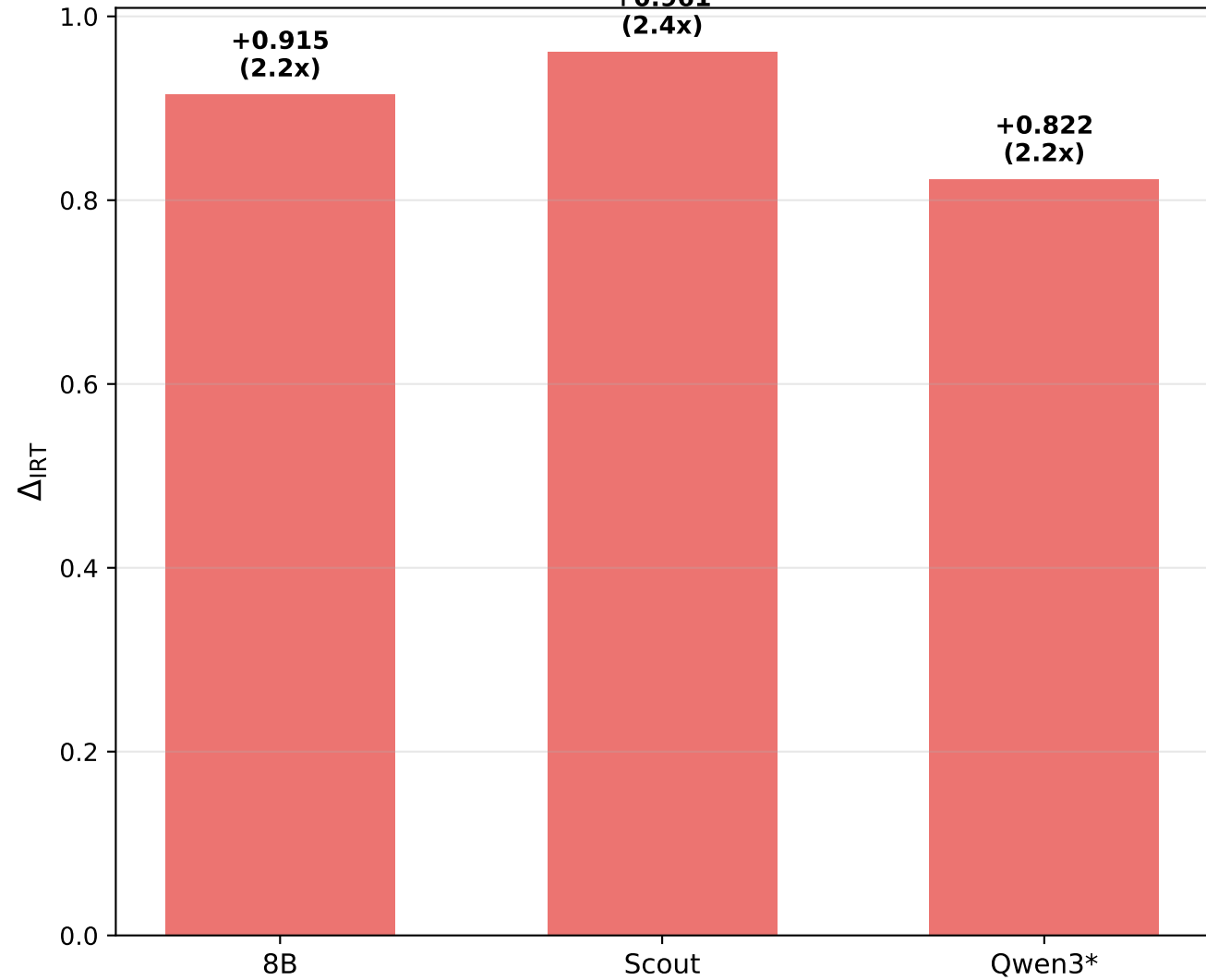
(B) IRT-Weighted Delta (Amplification Factor)
