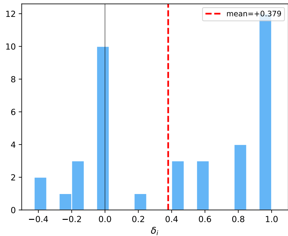
Qwen3 (partial) N=41
