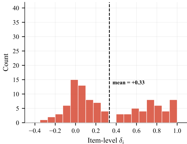
A. Pre-verification (N=100) Bimodal: broken items inflate mean
