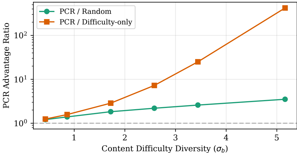
PCR Advantage Scales with Difficulty Diversity
