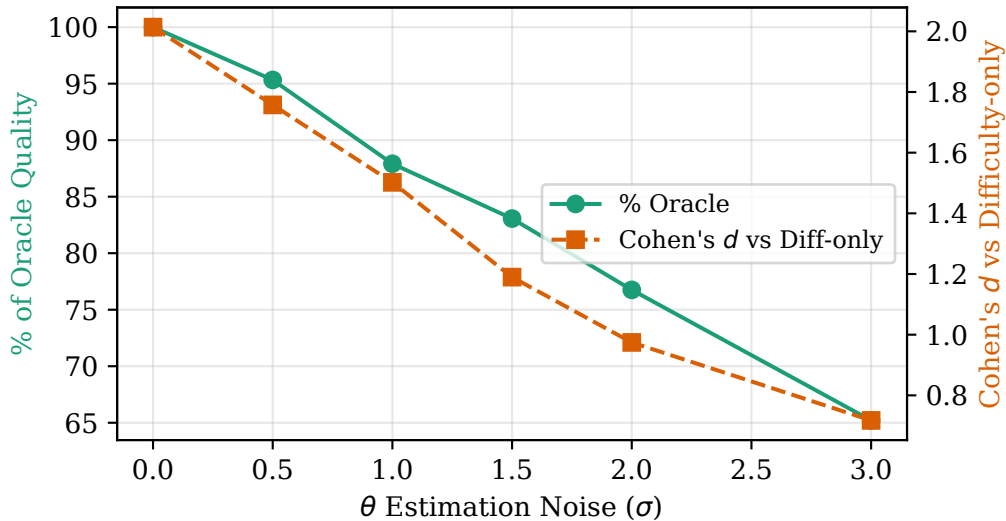
Robustness to \theta Estimation Noise
