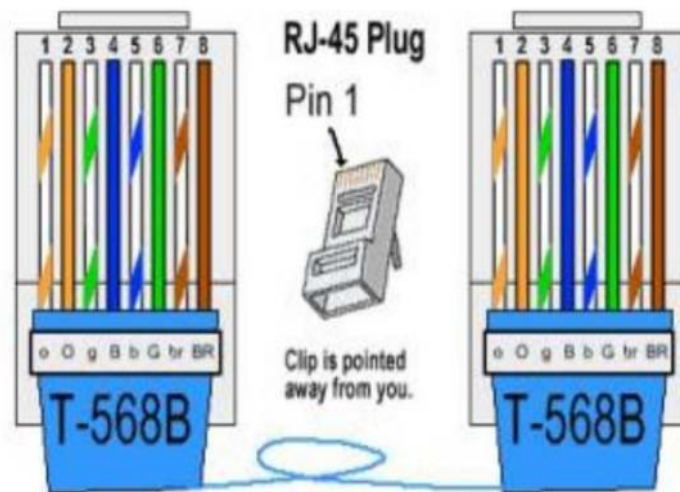
Straight-Through Ethernet Cable
