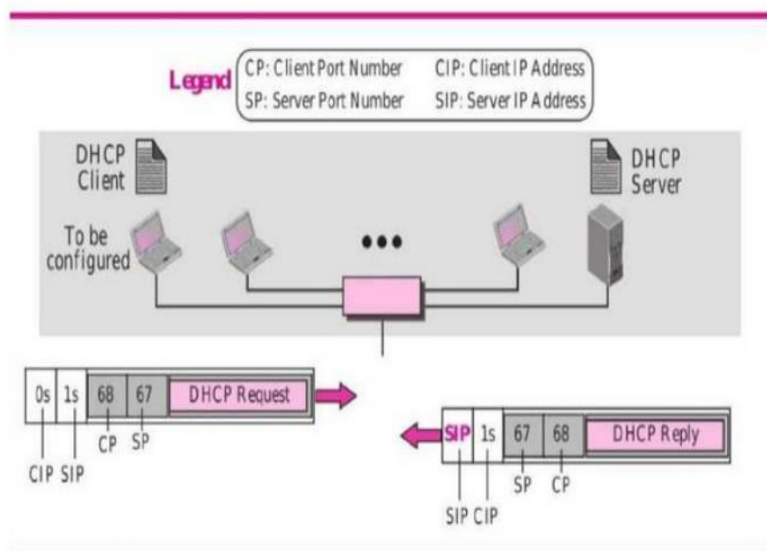
Figure 1: Client and server on the same network
