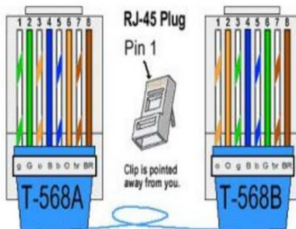
Straight-Through Ethernet Cable
