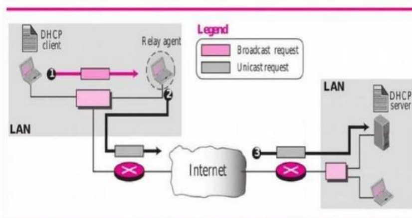
Figure 2 : Client and server on two different networks
