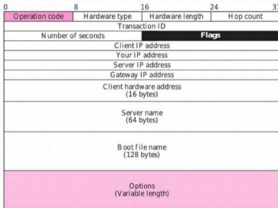
Figure 3 :DHCP packet format
