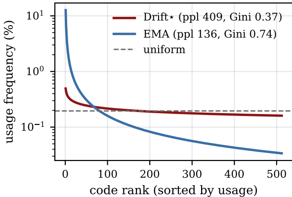
Codebook usage (CIFAR-10, K = 512 )
