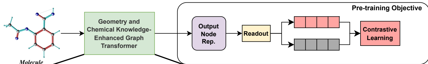
(A) Overall Pre-training Framework
