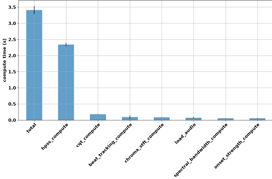
Figure 1: The computational time (in seconds) averaged on 200 audio tracks for the 7 most time consuming features. The total bar gives the average total computational time for one track.
