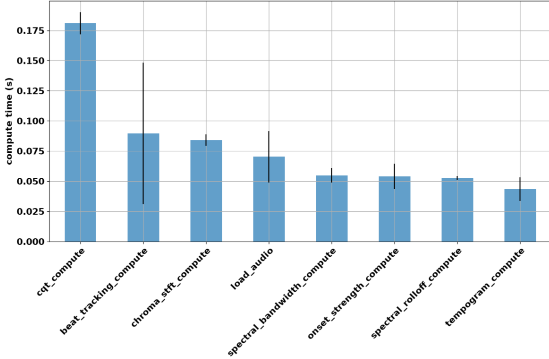
Figure 2: The computational time (in seconds) averaged on 200 audio tracks for the most time consuming features. The bars for total and hpss_compute have been removed to better see the variations on the next columns.
