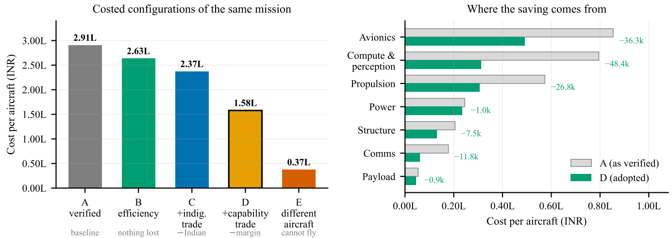
Fig. 9. Costed configurations, ordered by what each trades away. A through D are the same aircraft; E is a different and much smaller airframe that cannot carry the payload, included to show where the cost floor genuinely lies rather than as a proposal. Option D is adopted: it gives up margin and indigenous content, but no scored capability.
