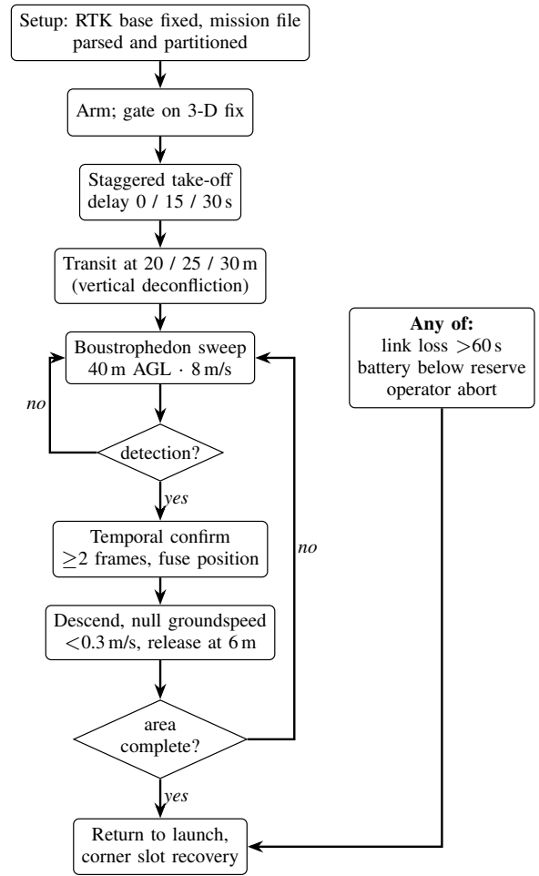
Fig. 2. Autonomous mission sequence. The take-off stagger is encoded in the mission file rather than in operator timing, and all three abnormal conditions converge on a single return-to-launch path.
