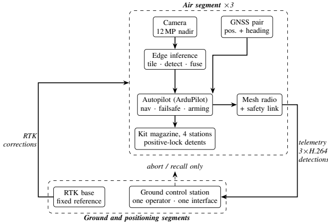
Fig. 1. System architecture. The only permitted downlink commands are abort and recall; the ground station is architecturally incapable of originating a retask, waypoint change or drop command. Detection runs onboard, so the downlink serves the operator rather than the algorithm.
