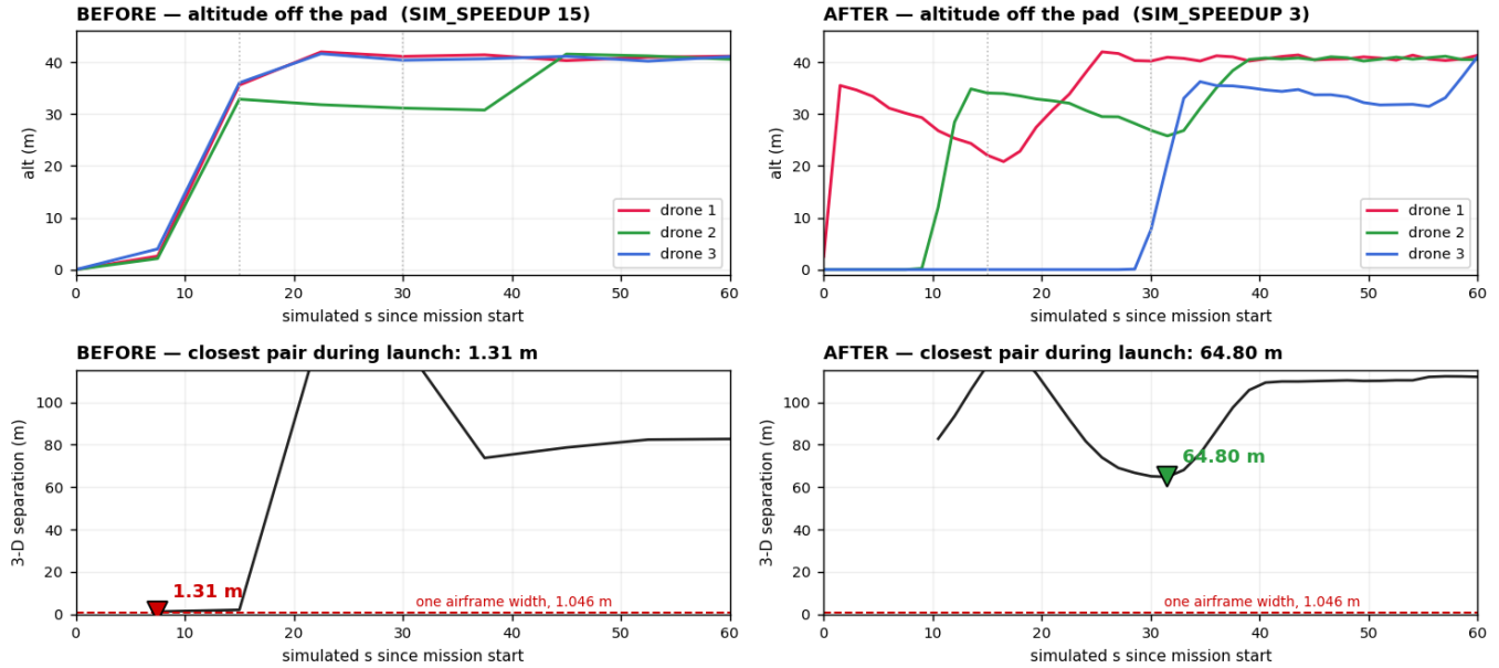
Fig. 3. Launch deconfliction, recorded from three ArduCopter software-in-the-loop autopilots. Left: all three aircraft leave the pad together and the closest pair passes within 1.31 m — inside one airframe width. Right: a delay encoded in the mission file before each take-off command staggers them, and the closest airborne pair is 64.80 m. Both figures are reproducible from the committed telemetry.
