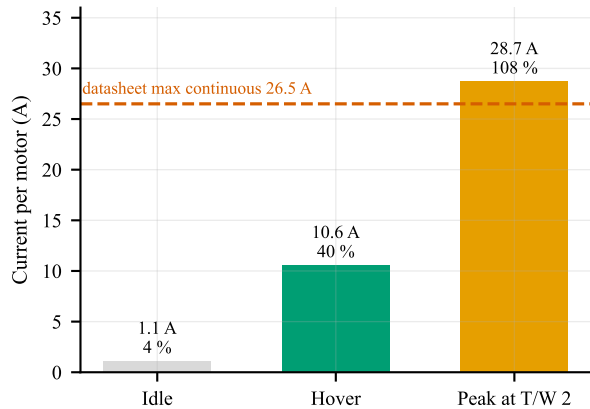
(b) Tarot TL96020 operating point
