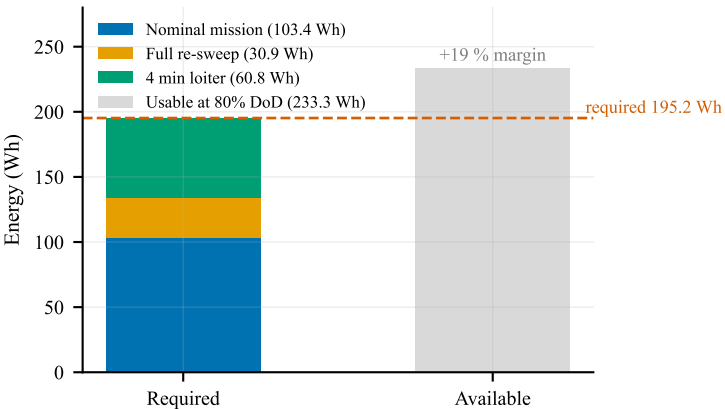
(a) Reserve policy against pack capacity
