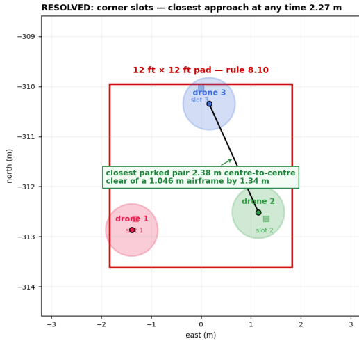
A ROW of three gave 1.22 m spacing and they landed 0.83 m apart — an overlap of 1.046 m airframes. Centres must stay half an airframe inside the pad edge, so they live in a 2.61 m square; its CORNERS are 2.61 m apart — two Worst case with \pm 0.5 m touchdown dispersion on each aircraft: 1.61 m, still clear. Holding over points 2.6 m apart instead of the stacked-over-the-pad separation from 3.99 m to 6.52 m.
