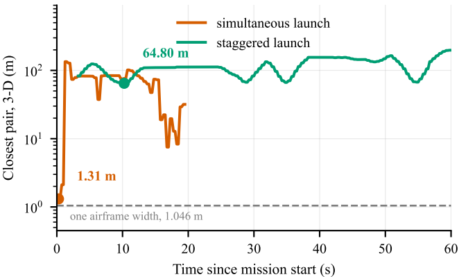
(a) Separation during launch
