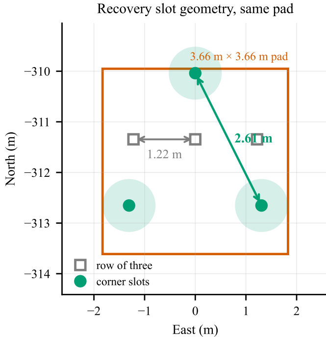
Fig. 6. Recovery slot geometry, drawn from the two committed recordings. Slot centres must stay half an airframe inside the pad edge, so they live in a 2.61 m square: a row across that square gives 1.22 m of spacing, its corners give the full 2.61 m. Shaded discs are the 1.046 m airframe footprint at the corner slots. The measured closest approach at any time rises from an overlapping 0.83 m to 2.27 m — twice the separation, on the same pad, at no cost.
