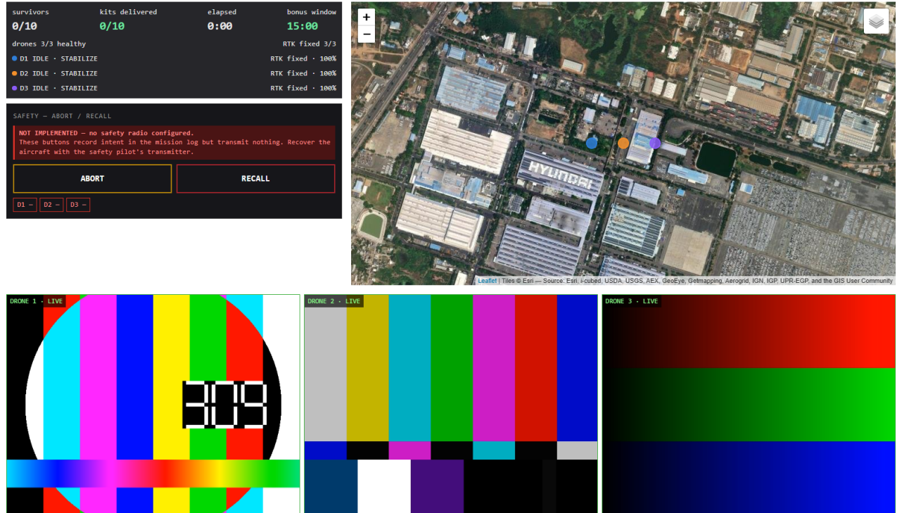
Fig. 9. Ground control station, captured unretouched from the running system. The interface carries mission status, per-aircraft mode, RTK fix state and battery, the shared map, kit-delivery count, and three concurrent H.264 feeds within the 2.5Mbps link budget. Map tiles are served from a local cache, so nothing here depends on a network. The 15:00 counter is the SYS-35 fast-completion threshold, half the permitted window, rather than the flight-time limit. This is a bench capture, not a mission. No mission file is loaded, which is why all three aircraft read STABILIZE at 100% charge, why no assigned search areas or survivor markers are drawn, and why the video panes carry test patterns; no camera has yet flown. The safety panel is shown uncropped deliberately: it states that abort and recall are not implemented , that they record operator intent in the mission log and transmit nothing, and that recovery is by the safety pilot's transmitter — because no downlink command path is yet wired. See Section VII-C.
