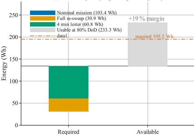
(a) Reserve policy against pack capacity
