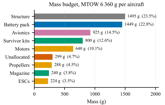
Fig. 1. Mass budget per aircraft. Generated from docs/sizing/model-output.txt. Avionics includes the wiring harness and magazine the release mechanism. The fleet figure of 19 081 g carries 4919 g of growth allowance against a 24 kg internal target — 26 % build overweight tolerated — inside the 25 kg regulatory cap.
