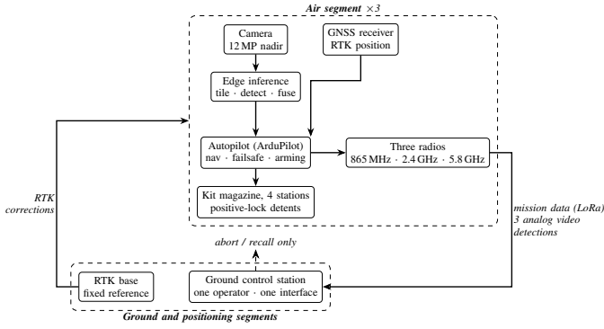
Fig. 4. System architecture. The only permitted downlink commands are abort and recall; the ground station is architecturally incapable of originating a retask, waypoint change or drop command. Detection runs onboard, so the downlink serves the operator rather than the algorithm.
