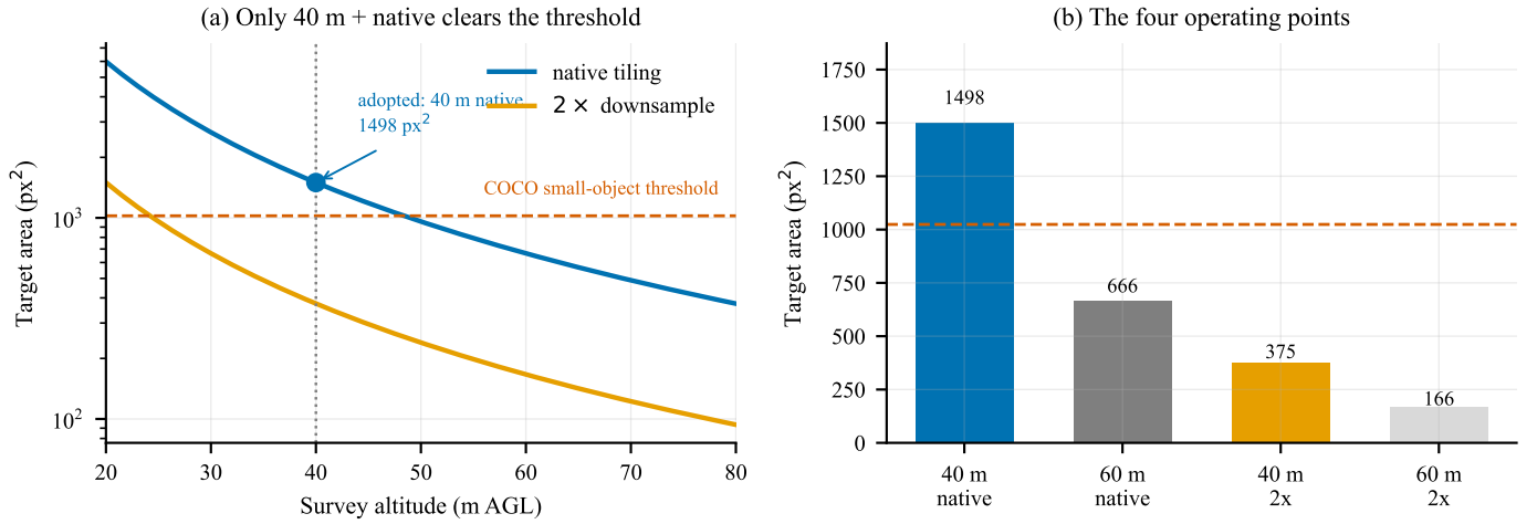
Fig. 8. Target area against survey altitude, for a person in water presenting head and shoulders. (a) Only the adopted point — 40 m with native-resolution tiling — sits above the COCO small-object threshold; downsampling by two drops it below at every altitude. (b) The four candidate operating points. The two changes are not independent: either one alone leaves the target in the size band where published detector accuracy collapses.
