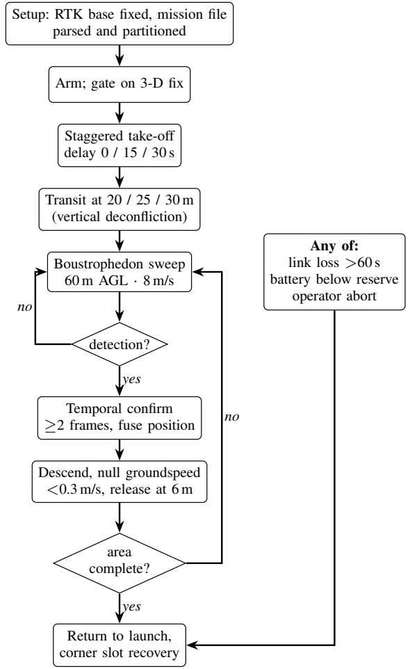
Fig. 11. Autonomous mission sequence. The take-off stagger is encoded in the mission file rather than in operator timing, and all three abnormal conditions converge on a single return-to-launch path.
