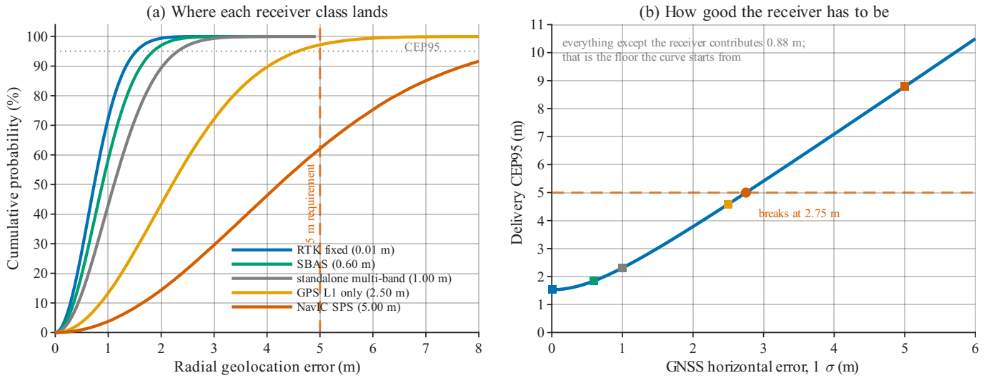
Fig. 5. (a) Radial error distribution for five receiver classes over the full geolocation budget, 200 000 Monte Carlo samples each. (b) The same result as a criterion: delivery CEP95 against the receiver's own horizontal error, with the 5 m requirement and the 2.75 m break point of (1). Markers are the five classes of panel (a) in the same colours. The curve does not start at zero — 0.88 m of the budget belongs to terms no receiver touches.
