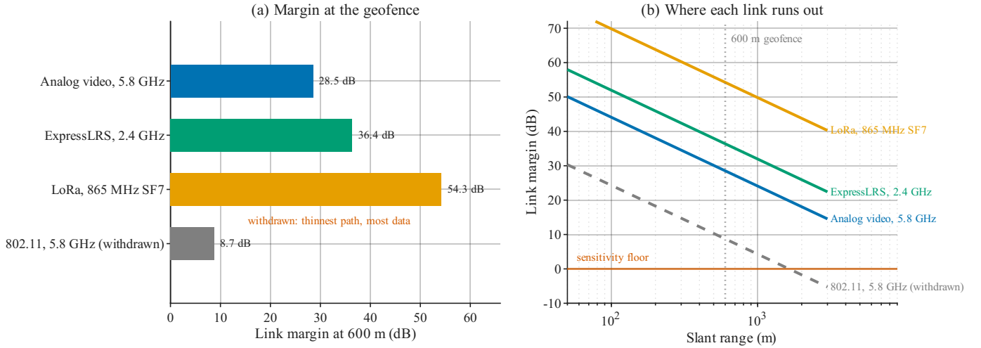
Fig. 12. (a) Link margin at the 600 m geofence, from (3). The withdrawn 802.11 mesh is retained in the figure because the withdrawal is an argument and the margin column is that argument. (b) Margin against slant range. Every adopted link is flown at a small fraction of the range at which it runs out; the withdrawn one is not.
