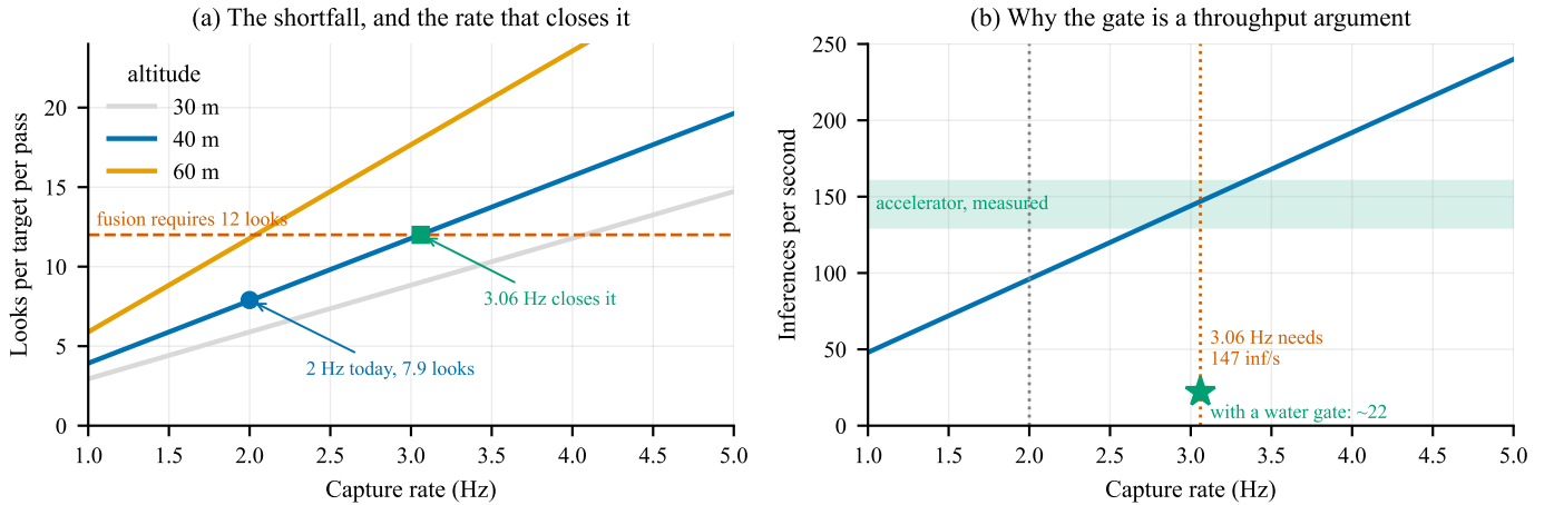
Fig. 9. (a) Looks per target per pass against capture rate. Multi-frame fusion requires twelve; the adopted 2 Hz supplies 7.9, and 3.06 Hz closes the gap. Lowering altitude worsens the shortfall rather than easing it, because the along-track footprint shrinks faster than the pass shortens. (b) What that rate costs. At 48 native tiles, 3.06 Hz is 147 inferences per second against the 130–160 measured for the accelerator — at or beyond the limit. A gate discarding the tiles that are open water is what buys it back, which makes the cascade a throughput argument rather than an accuracy one.
