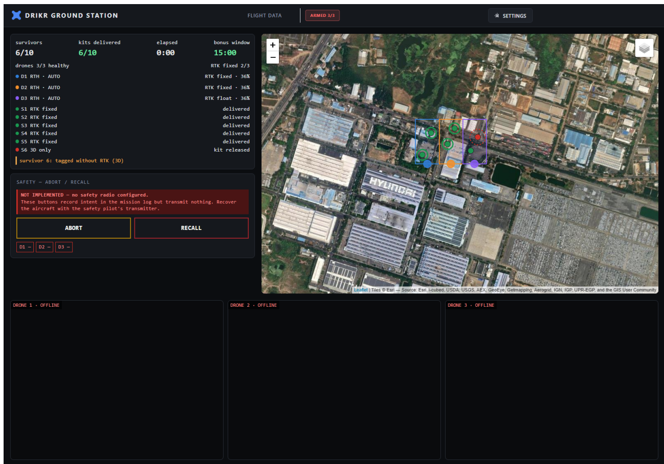
Fig. 16. Ground control station, captured unretouched from the running client and backend. The telemetry is synthetic: a mission driver ( scripts/sim_mission.py ) emits MAVLink and 5 Hz mission-state documents for three aircraft, so every display can be exercised before an aircraft exists. No aircraft, autopilot or radio is involved. Visible here: the three assigned search regions on a satellite basemap served from a local tile cache, so nothing depends on a network; three aircraft armed and in AUTO, two with an RTK-fixed solution and the third in float, which is the degraded case the display must distinguish; and the mission counters, where the 15:00 figure is the SYS-35 fast-completion threshold rather than the flight-time limit. The run is caught after delivery, with six survivors located and six kits released, which is what puts the per-survivor rows on screen. Those rows carry the point Section IV-D2 argues: five survivors are tagged RTK FIXED and the sixth 3D ONLY, and the display says so rather than presenting six coordinates of equal worth. A rescue coordinator acting on the sixth is working to a different radius than on the other five, and the interface is required to make that visible. The safety panel is shown uncropped deliberately. It states that abort and recall are not implemented , that they record operator intent in the mission log and transmit nothing, and that recovery is by the safety pilot's transmitter — because no downlink command path is yet wired (Section VII-C). The video panes read offline because the media server is not running in this capture; no camera has yet flown.
