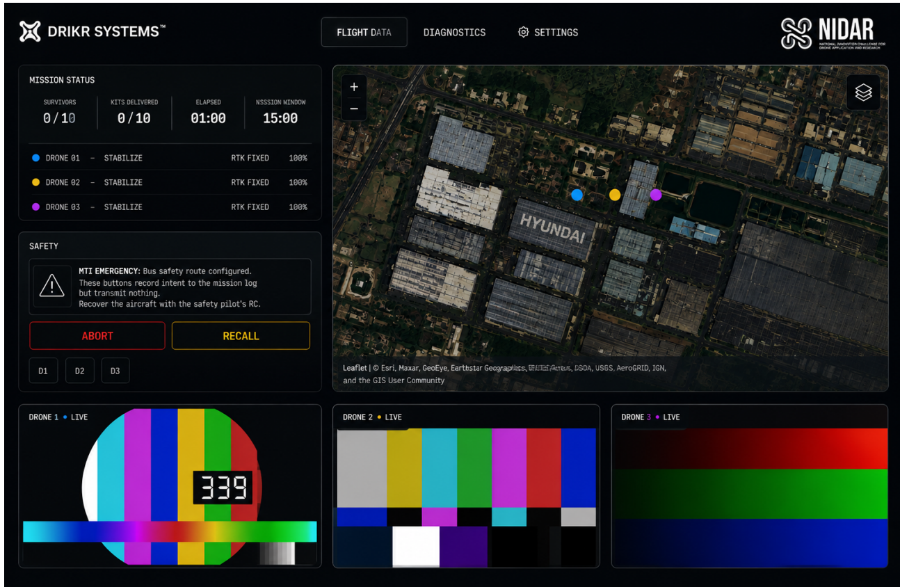
Fig. 8. Ground control station, captured from the running system. A single operator interface carries all eight displays the rules require: mission status, per-aircraft mode, RTK fix state and battery, the shared map, and three concurrent H.264 feeds within the 2.5 Mbps link budget. Map tiles are served from a local cache, so nothing here depends on a network. The safety panel is shown uncropped : abort and recall record operator intent in the mission log and transmit nothing, because no downlink command path is yet wired — see Section VI-C. The video panes carry test patterns; no camera has yet flown.
