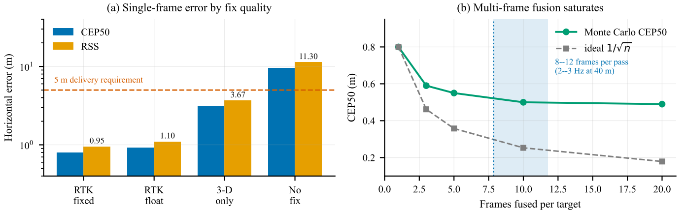
Fig. 6. Geolocation error, from a Monte Carlo run through the same projection code the aircraft flies. (a) Single-frame horizontal error against GNSS fix quality, typical attitude, on a logarithmic scale; the dashed line is the 5 m delivery requirement. (b) Effect of fusing multiple observations of the same target, RTK fixed. Generated by figures/make_figures.py from docs/sizing/geotag-accuracy-output.txt .
