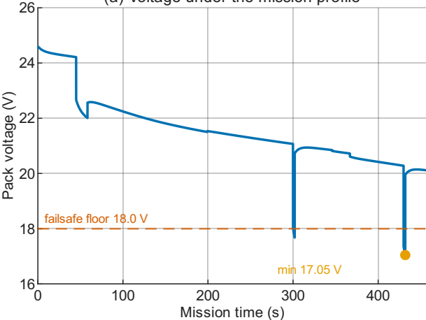
(a) Voltage under the mission profile
