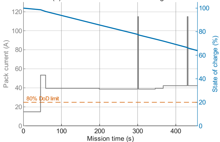
(b) Current draw and state of charge
