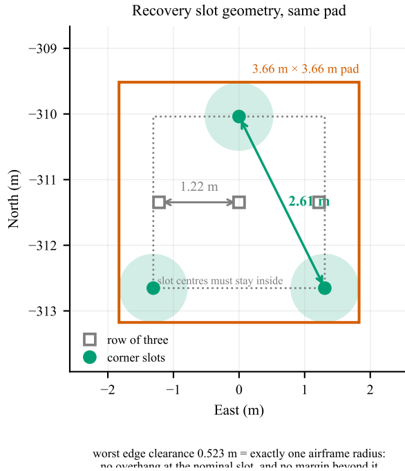
Fig. 12. Recovery slot geometry, drawn from the two committed recordings. Slot centres must stay half an airframe inside the pad edge, so they live in a 2.61 m square: a row across that square gives 1.22 m of spacing, its corners give the full 2.61 m. Shaded discs are the 1.046 m airframe footprint at the corner slots. The measured closest approach at any time rises from an overlapping 0.83 m to 2.27 m — twice the separation, on the same pad, at no cost.
