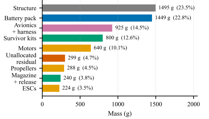
Fig. 1. Mass budget per aircraft. Generated from docs/sizing/model-output.txt. The fleet figure of 19 081 g carries 4919 g of growth allowance against a 24 kg internal target — 26 % build overweight tolerated — inside the 25 kg regulatory cap.
