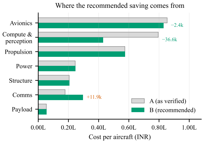
Fig. 10. Subsystem cost, Option A against Option B. Almost the whole saving is one substitution in compute and perception. Communications moves the other way: the sub-gigahertz safety link is corrected upward by INR 11 855, because the carried figure does not buy a compliant radio.
