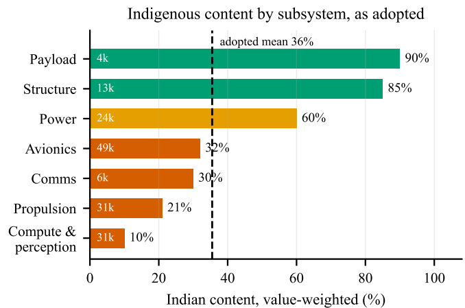
Fig. 12. Indian content by subsystem for the adopted configuration, value-weighted, with subsystem cost annotated inside each bar. Four subsystems now sit below 40 %, and between them they carry INR 1.17 L of the INR 1.58 L aircraft — which is why the aggregate is worth decomposing rather than quoting alone. What remains strongly domestic is what the team fabricates itself.
