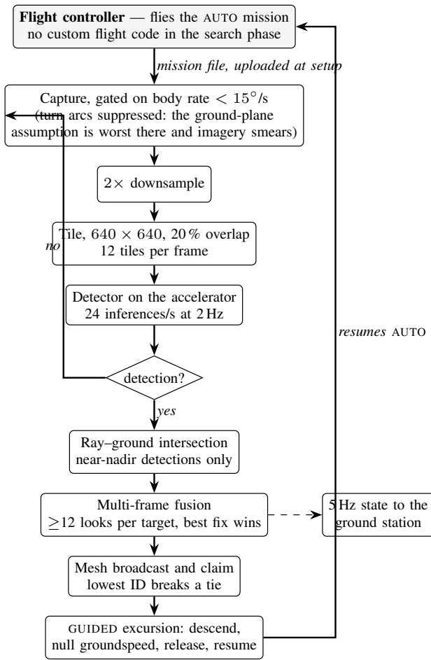
Fig. 4. Onboard processing. The autopilot flies the search pattern unaided; the companion computer detects, geolocates and claims survivors, and interrupts the mission only to deliver. Detection runs alongside the sweep and never gates it — a missed frame costs a look, not a waypoint.
