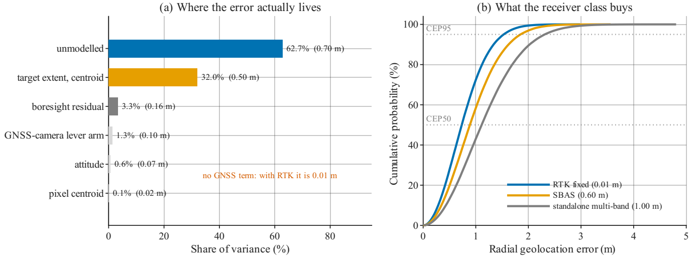
Fig. 5. (a) Where the geolocation error actually lives. Unmodelled error and target centroid carry 95 % of the variance, and there is no GNSS position term at all — with RTK it is 1 cm. (b) Radial error distribution by receiver class, 200 000 Monte Carlo samples over the full budget. The separation between an RTK receiver and an SBAS one is 0.16 m of CEP50, against terms neither can reduce.
