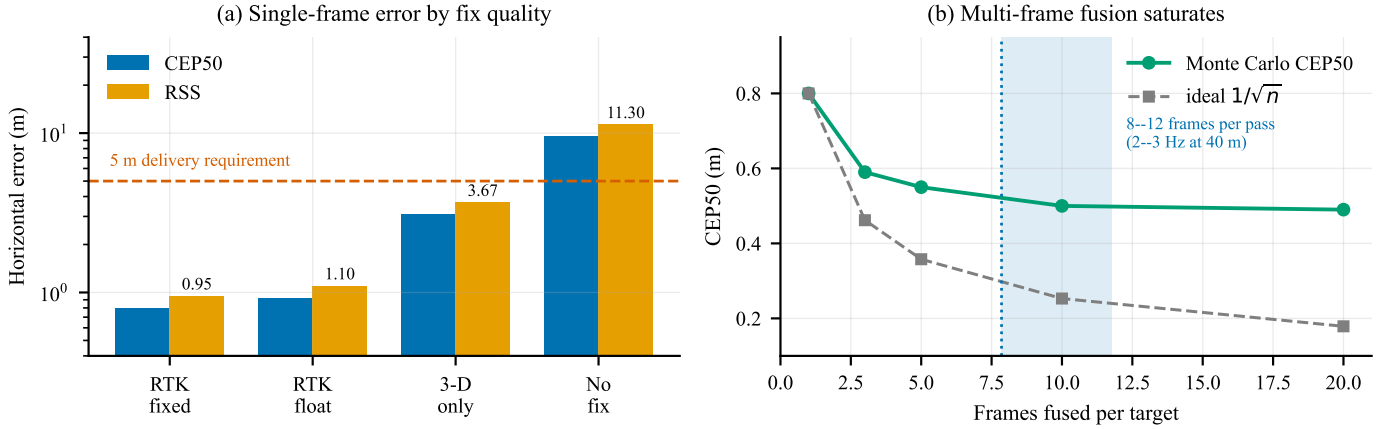
Fig. 6. Geolocation error, from a Monte Carlo run through the same projection code the aircraft flies. (a) Single-frame horizontal error against GNSS fix quality, typical attitude, on a logarithmic scale; the dashed line is the 5 m delivery requirement. (b) Effect of fusing multiple observations of the same target, RTK fixed. Generated by figures/make_figures.py from docs/sizing/geotag-accuracy-output.txt .
