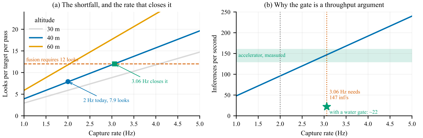
Fig. 8. (a) Looks per target per pass against capture rate. Multi-frame fusion requires twelve; the adopted 2 Hz supplies 7.9, and 3.06 Hz closes the gap. Lowering altitude worsens the shortfall rather than easing it, because the along-track footprint shrinks faster than the pass shortens. (b) What that rate costs. At 48 native tiles, 3.06 Hz is 147 inferences per second against the 130–160 measured for the accelerator — at or beyond the limit. A gate discarding the tiles that are open water is what buys it back, which makes the cascade a throughput argument rather than an accuracy one.
