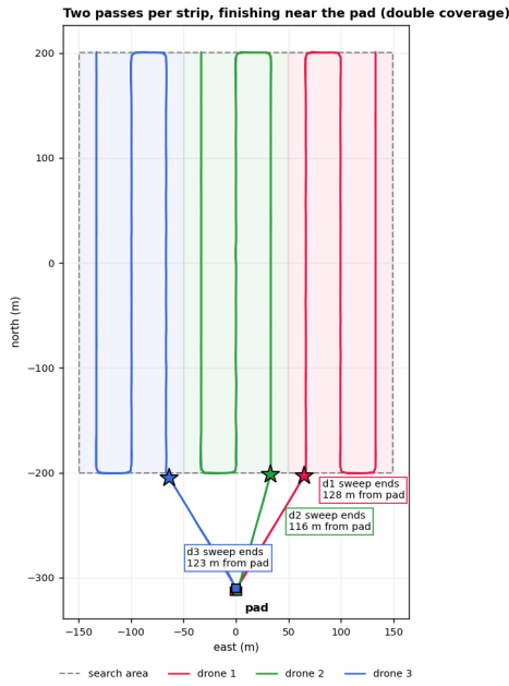
Each strip is swept TWICE — the second pass retraces the same ground on the reverse heading, so the two overlap here. The evidence 18/19/19 items against 12/13/13 for a single pass, and 2535 m of path against 1267 m. It is for the GEOTAG, not coverage: boresight systematic and only cancels when the same ground is seen from the opposite direction. The cost is a second sweep, 347 s against 1 Sweep also finish near the pad now — 116–123 m, against 516 m and 540 m for two of three aircraft before.
