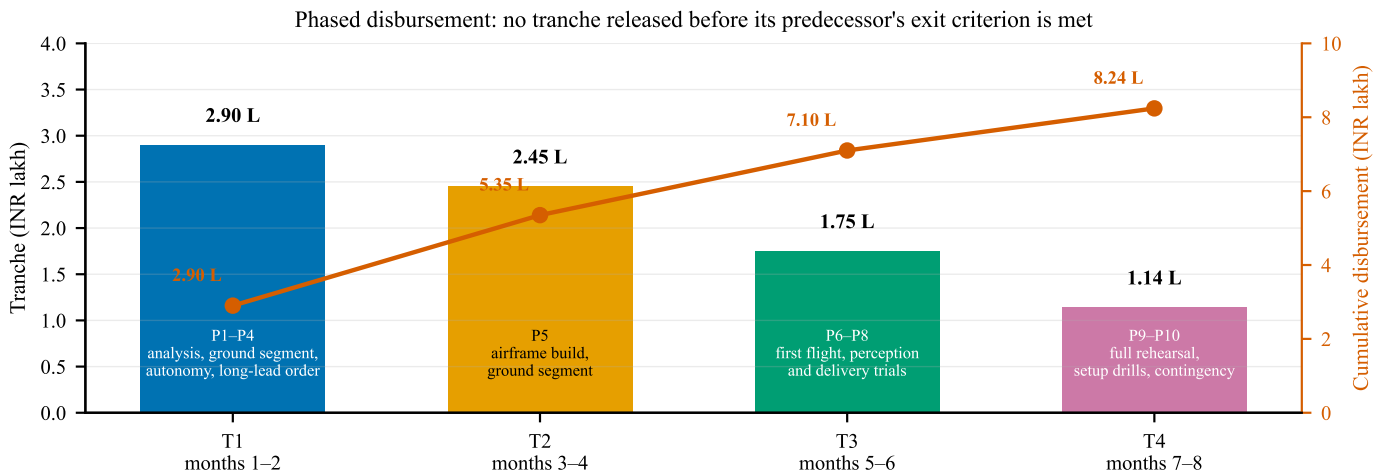
Fig. 10. Phased disbursement against programme phases. Tranche 1 is front-loaded because long-lead components must be ordered in month one for the eight-week flight-test window to survive; tranche 4 is the smallest and carries the contingency.
