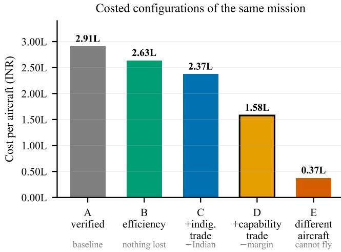
Fig. 9. Costed configurations, ordered by what each trades away. A through D are the same aircraft; E is a different and much smaller aircraft that cannot carry the payload, included to show where the cost floor genuinely lies rather than as a proposal. Option D is adopted: it gives up margin and indigenous content, but no scored capability.
