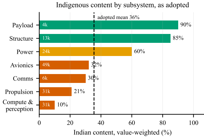
Fig. 11. Indian content by subsystem for the adopted configuration, value-weighted, with subsystem cost annotated inside each bar. Four subsystems now sit below 40 %, and between them they carry INR 1.17 L of the INR 1.58 L aircraft — which is why the aggregate is worth decomposing rather than quoting alone. What remains strongly domestic is what the team fabricates itself.
