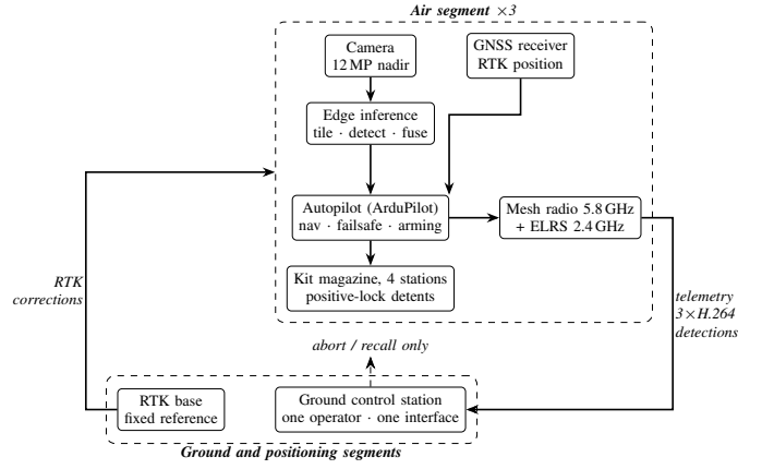
Fig. 2. System architecture. The only permitted downlink commands are abort and recall; the ground station is architecturally incapable of originating a retask, waypoint change or drop command. Detection runs onboard, so the downlink serves the operator rather than the algorithm.
