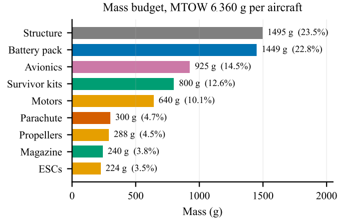
Fig. 1. Mass budget per aircraft. Generated from docs/sizing/model-output.txt. Avionics includes the wiring harness and magazine the release mechanism. The fleet figure of 19081 g carries 4919 g of growth allowance against a 24 kg internal target — 26 % build overweight tolerated — inside the 25 kg regulatory cap.
