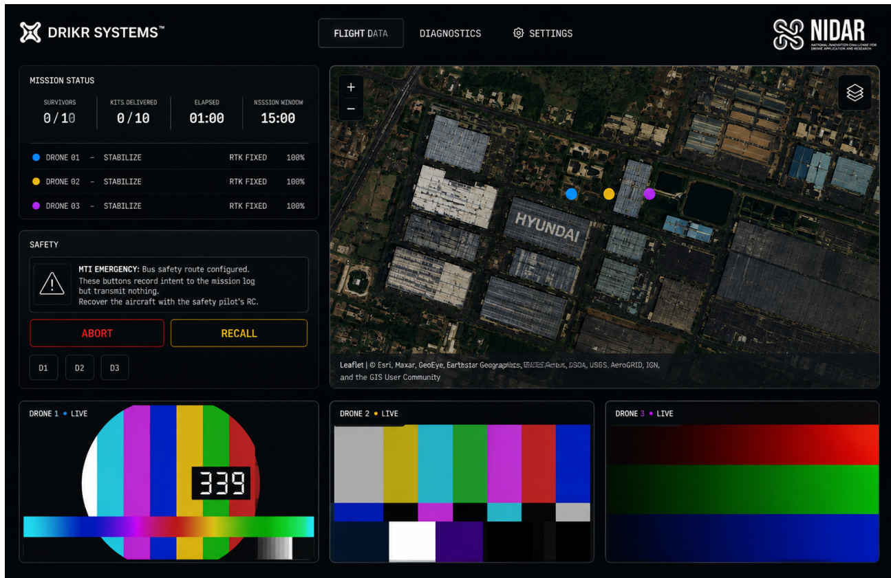
Fig. 9. Ground control station, captured from the running system and shown unretouched . The interface carries mission status, per-aircraft mode, RTK fix state and battery, the shared map, kit-delivery count, and three concurrent H.264 feeds within the 2.5Mbps link budget. Map tiles are served from a local cache, so nothing here depends on a network. The mission counters are correct: rule 8.11 caps survivors at ten, and the 15:00 window is the SYS-35 fast-completion threshold — half the permitted thirty minutes — rather than the flight-time limit. This is a bench capture, not a mission. No mission file is loaded, which is why all three aircraft read STABILIZE at 100% charge, why no assigned search areas or survivor markers are drawn, and why the video panes carry test patterns; no camera has yet flown. Two strings in the interface are wrong and are visible here: the header reads NSSSION WINDOW for MISSION WINDOW, and the safety banner reads MTI EMERGENCY: Bus safety route configured, which is garbled — the previous build read NOT IMPLEMENTED --- no safety radio configured, which is what is actually true. Both are fixed in the interface repository, not here. The rest of that panel is correct and is the reason it is shown uncropped: abort and recall record operator intent in the mission log and transmit nothing, because no downlink command path is yet wired — see Section VII-C.
