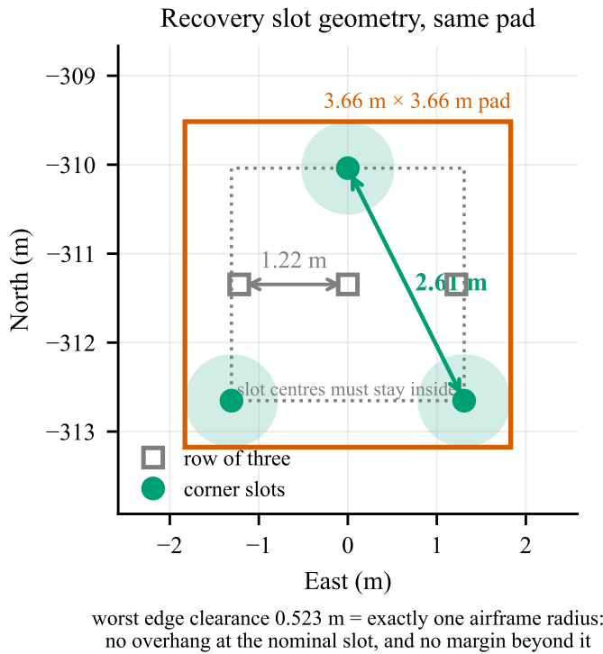
Fig. 6. Recovery slot geometry, drawn from the two committed recordings. Slot centres must stay half an airframe inside the pad edge, so they live in a 2.61 m square; a row across that square gives 1.22 m of spacing, its corners give the full 2.61 m. Shaded discs are the 1.046 m airframe footprint at the corner slots. The measured closest approach at any time rises from an overlapping 0.83 m to 2.27 m — twice the separation, on the same pad, at no cost.
