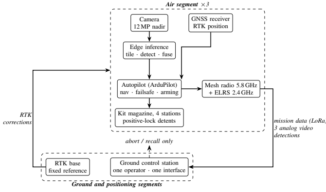
Fig. 4. System architecture. The only permitted downlink commands are abort and recall; the ground station is architecturally incapable of originating a retask, waypoint change or drop command. Detection runs onboard, so the downlink serves the operator rather than the algorithm.
