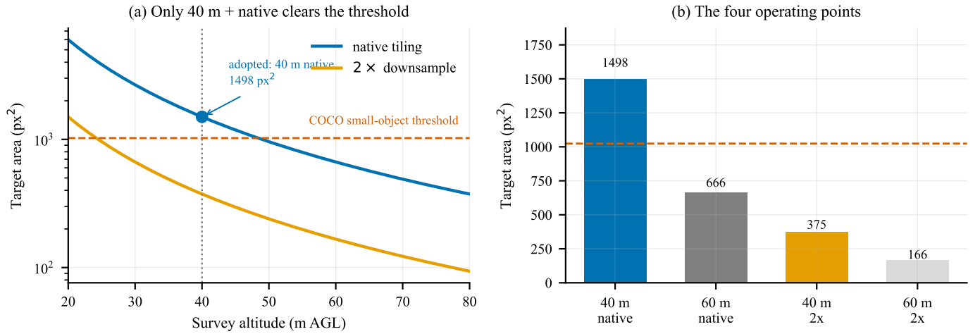
Fig. 6. Target area against survey altitude, for a person in water presenting head and shoulders. (a) Only the adopted point — 40 m with native-resolution tiling — sits above the COCO small-object threshold; downsampling by two drops it below at every altitude. (b) The four candidate operating points. The two changes are not independent: either one alone leaves the target in the size band where published detector accuracy collapses.
