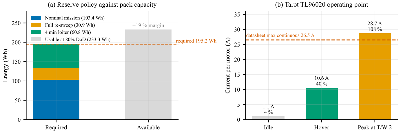
Fig. 2. (a) The reserve policy against what the pack delivers: the nominal mission, a full second sweep of the search area and four minutes of loiter, all inside the 80 % usable window. (b) The selected motor against its own datasheet. Hover sits at 40 % of rated continuous current with wide margin; the peak at the design thrust-to-weight sits at 108 %, which is acceptable only because T/W = 2 is a transient authority reserve rather than a flight condition. It is the tightest margin in the propulsion chain, and P2 measures current alongside thrust to settle it.
