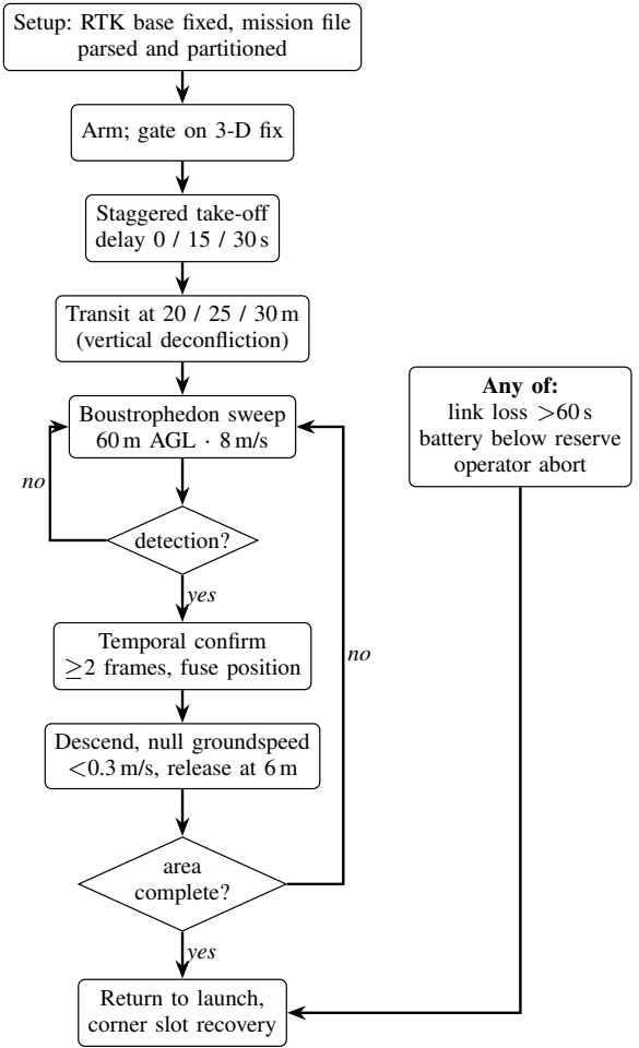
Fig. 9. Autonomous mission sequence. The take-off stagger is encoded in the mission file rather than in operator timing, and all three abnormal conditions converge on a single return-to-launch path.
