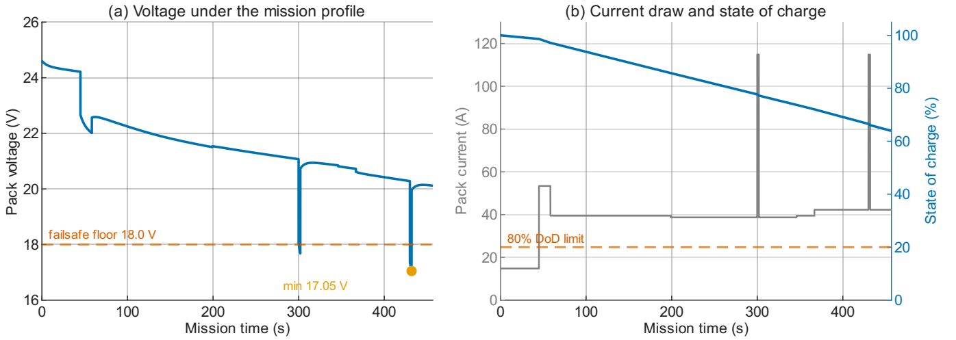
Fig. 3. Pack voltage under the mission profile, simulated with a second-order Thevenin cell model driven by the flight's own current trace and two gust-recovery transients at T/W = 2 . The pack reaches 17.05 V — below its own 18.0 V failsafe floor — at two-thirds state of charge, long before the 80 % depth-of-discharge limit the reserve policy is built around, and the dynamic sag exceeds the static estimate by 1.2 V because the diffusion terms add to the instantaneous ohmic drop. A failsafe set on instantaneous pack voltage would therefore command a return-to-land on a healthy pack mid-search. The internal resistance is calibrated to the static assumption rather than measured; P2 replaces it with a measured value.
