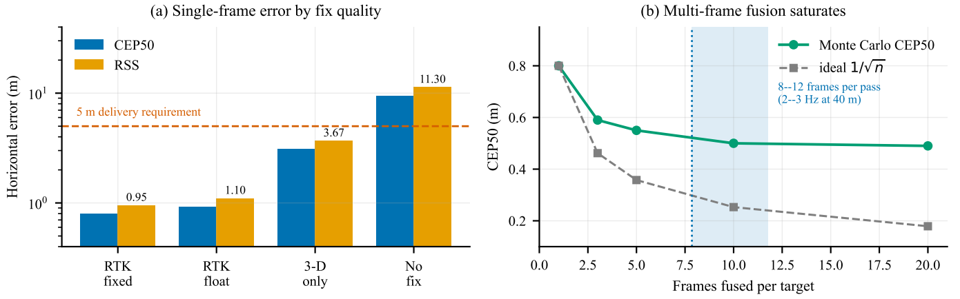
Fig. 5. Geolocation error, from a Monte Carlo run through the same projection code the aircraft flies. (a) Single-frame horizontal error against GNSS fix quality, typical attitude, on a logarithmic scale; the dashed line is the 5 m delivery requirement. (b) Effect of fusing multiple observations of the same target, RTK fixed. Generated by figures/make_figures.py from docs/sizing/geotag-accuracy-output.txt.
