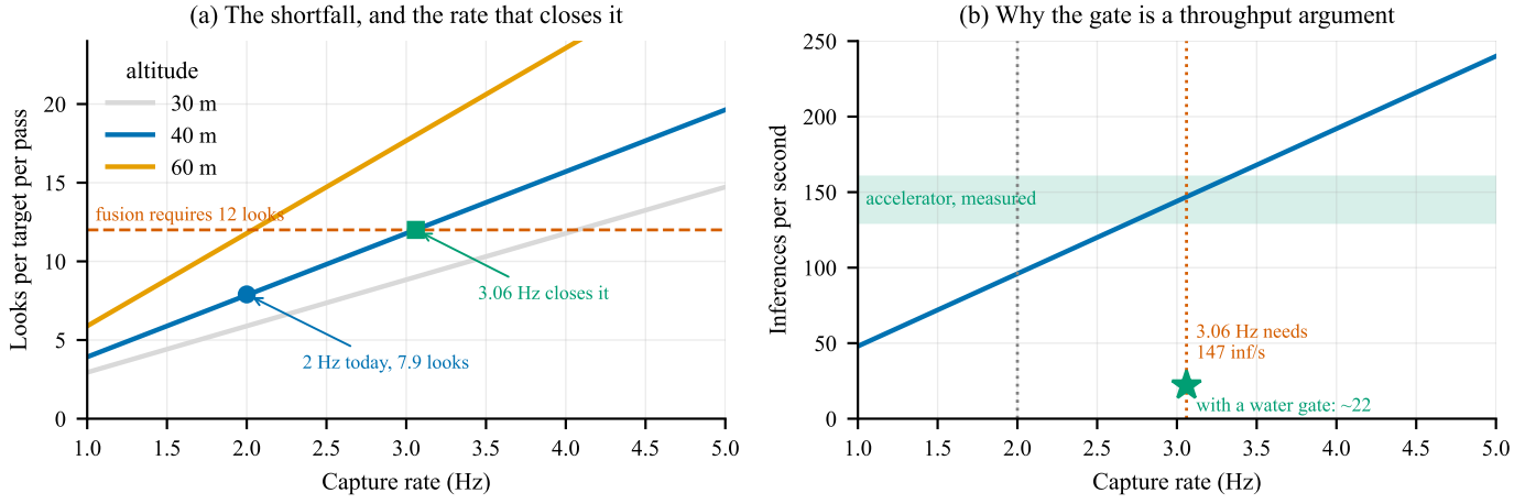
Fig. 7. (a) Looks per target per pass against capture rate. Multi-frame fusion requires twelve; the adopted 2 Hz supplies 7.9, and 3.06 Hz closes the gap. Lowering altitude worsens the shortfall rather than easing it, because the along-track footprint shrinks faster than the pass shortens. (b) What that rate costs. At 48 native tiles, 3.06 Hz is 147 inferences per second against the 130–160 measured for the accelerator — at or beyond the limit. A gate discarding the tiles that are open water is what buys it back, which makes the cascade a throughput argument rather than an accuracy one.
