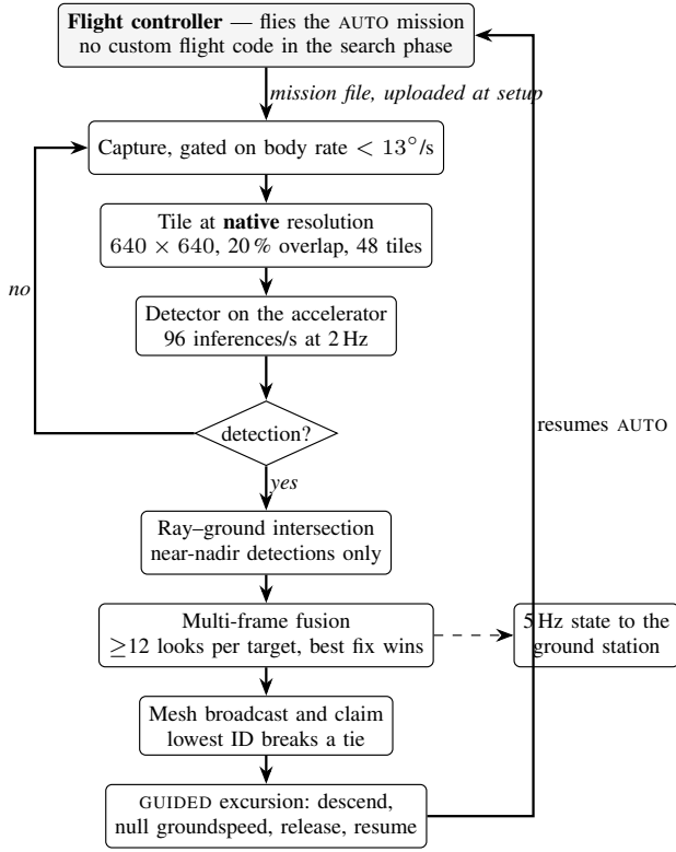
Fig. 8. Onboard processing. The autopilot flies the search pattern unaided; the companion computer detects, geolocates and claims survivors, and interrupts the mission only to deliver. Detection runs alongside the sweep and never gates it — a missed frame costs a look, not a waypoint. The capture gate suppresses turn arcs, where the ground-plane assumption is least valid and angular smear is worst. One pixel subtends 13.63 mdeg on this sensor, so at 1/1000 s a body rate of 13.6°/s is exactly one pixel of angular blur; the gate is set at 13°/s to sit under it.
