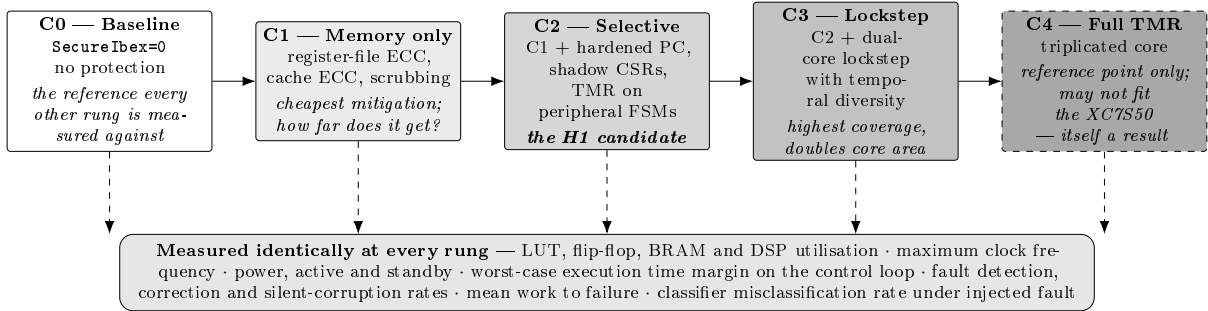
Figure 7: The configuration ladder. Ibex’s parameters make the independent variable genuinely independent: the same RTL, the same workload and the same fault schedule, with one protection mechanism added per rung. H1 predicts that C2 approaches C3’s mean work to failure at substantially lower cost, and that C4 either fails to fit or violates the control loop’s real-time deadlines — in which case that is a finding rather than a failure.
