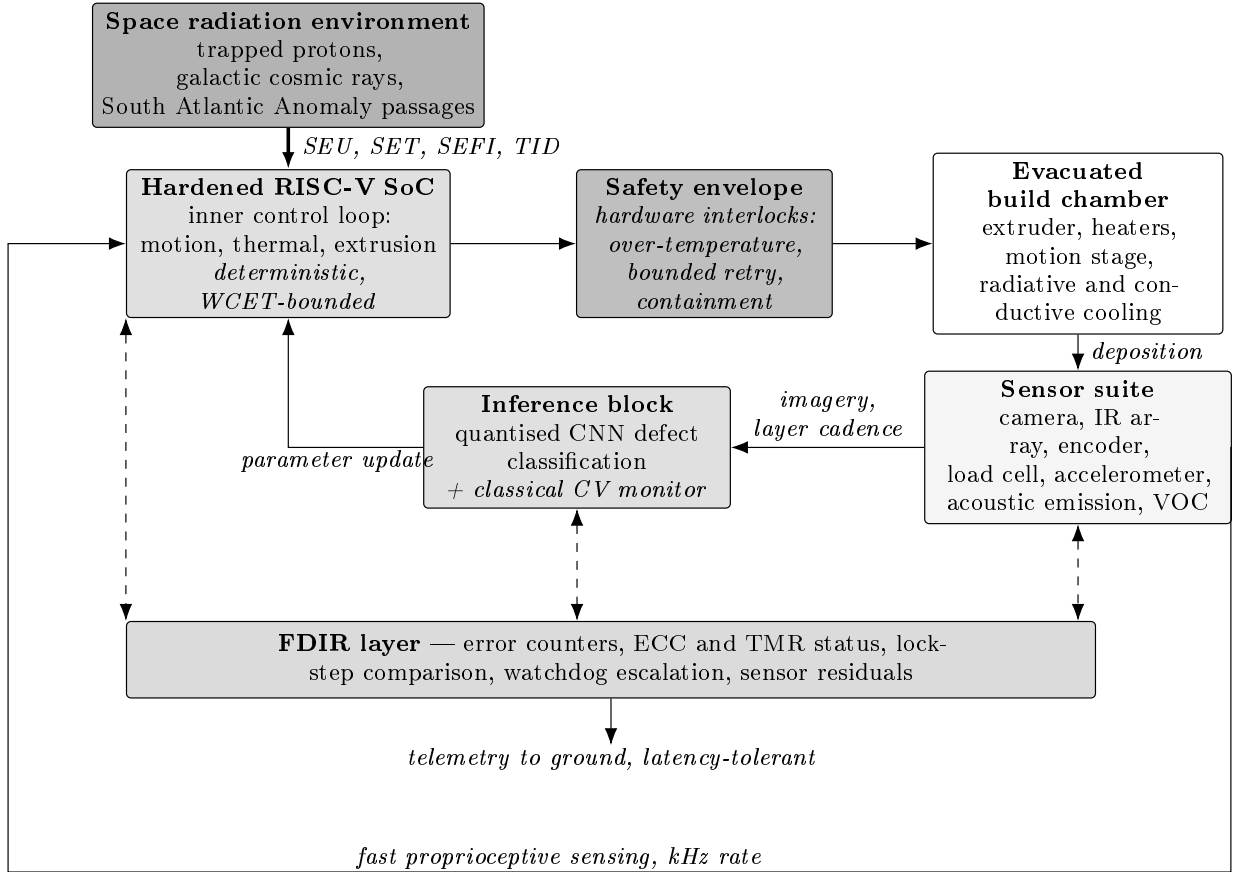
Figure 4: End-to-end system pipeline. Radiation acts on the controller, not on the process: charged particles upset the SoC, whose corrupted output then propagates forward through the safety envelope into the physical build, and returns through the sensor suite. Two return paths operate at different rates — fast proprioceptive sensing closes the inner control loop, while imagery closes the slower inspection loop through the inference block. The FDIR layer observes all three stages, which is what makes fault-origin discrimination (RQ3) possible at all.
