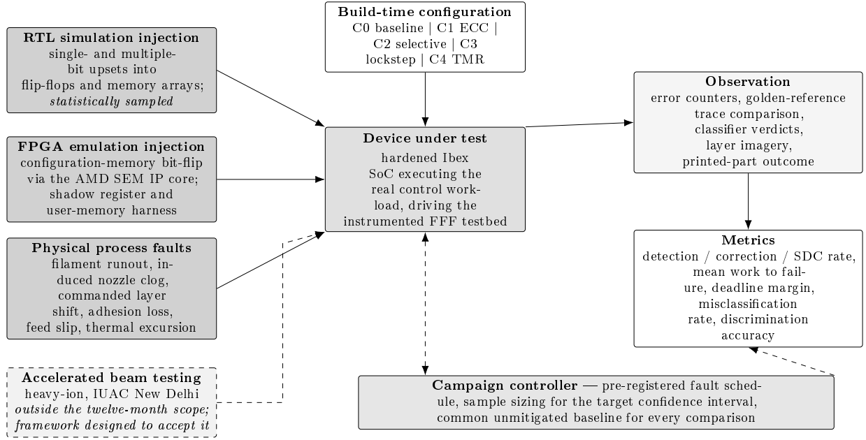
Figure 9: Fault-injection framework. Three injection routes drive a single device under test whose mitigations are selected at build time, so that every configuration is compared against a common unmitigated baseline under an identical, pre-registered fault schedule. The framework is deliberately structured so that accelerated beam testing can be added later as a fourth injection route without altering the measurement or analysis path.
