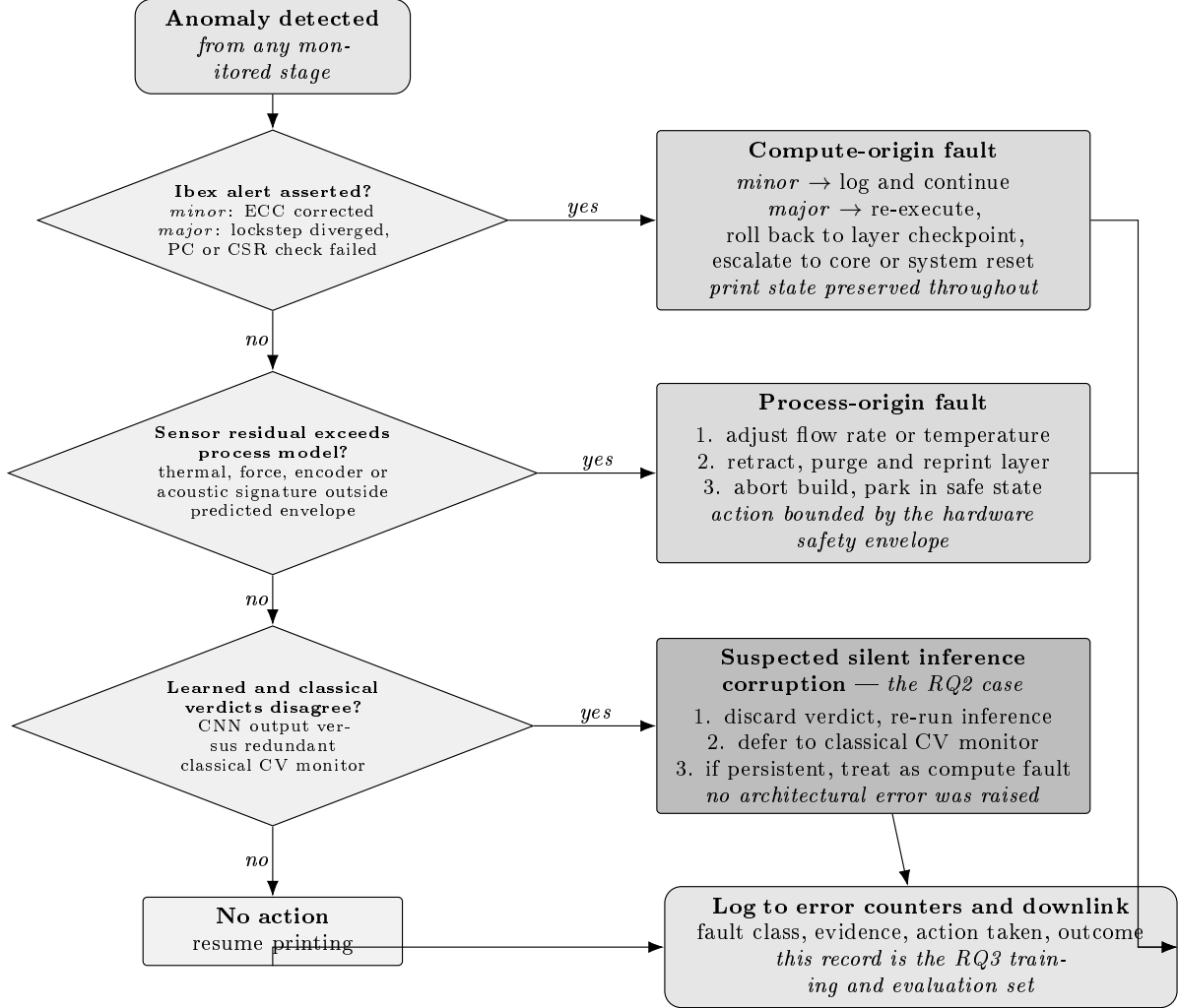
Figure 8: Fault detection, discrimination and recovery. The ordering of the tests is deliberate: an Ibex alert is unambiguous and is therefore checked first, and its minor/major distinction already separates corrected from uncorrectable faults. Process faults, by contrast, must be inferred from sensor residuals against a model. The third test exists only because of Gap 2 — an upset in the inference path raises no error signal and produces no residual anomaly, so the only remaining evidence is disagreement between the learned and classical verdicts. RQ3 asks how reliably the second and third branches can be separated from the first.
