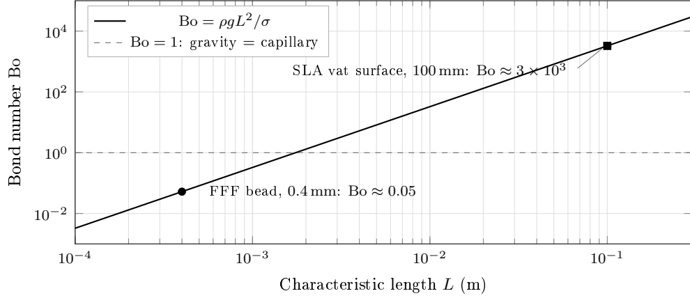
Figure 1: How much gravity matters, as a function of size, for molten plastic ( \rho = 1000 \text{ kg/m}^3 , \sigma = 0.03 \text{ N/m} ). Below the dashed line, surface tension wins and gravity is negligible. A printed bead sits well below it even on Earth, which is why extrusion still works in orbit. The open surface of a resin tank sits far above it, which is why resin printers do not.
