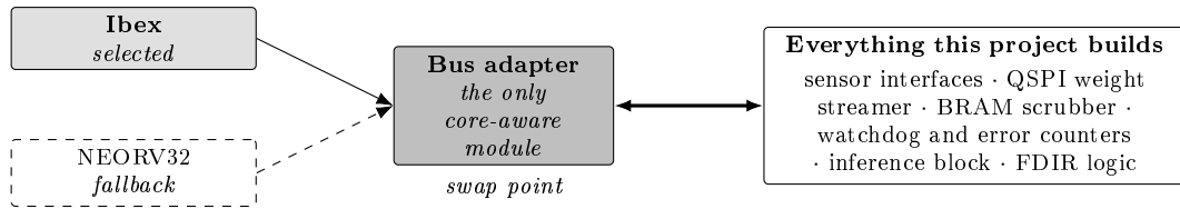
Figure 5: The bus adapter confines core-specific logic to one module. Switching base cores means rewriting the adapter, not the system: an estimated few days rather than the months a full re-integration would cost. This is what makes the NEORV32 fallback in Table 4 a genuine option rather than a formality.
