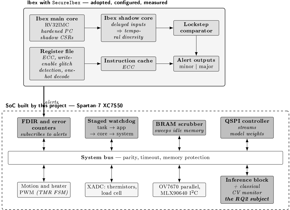
Figure 6: System architecture, drawn to separate what is adopted from what is built. The solid box is Ibex with SecureIbex enabled: lockstep with temporal diversity, register-file and cache ECC, hardened PC and shadow CSRs, all existing and all exposed through two alert lines. The dashed box is the SoC this project builds around it, including every mechanism Ibex does not provide — scrubbing, watchdog escalation, error-counter telemetry, TMR on peripheral control logic, and the inference path whose corruption is the subject of RQ2. Ibex supplies the signalling layer; the contribution is what subscribes to it.
