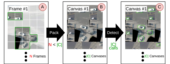
Figure 4: A video frame divided into a grid of tiles. Relevant tiles (highlighted) contain objects of interest, while irrelevant tiles (grayed) are discarded to save computation. Connected relevant tiles form a polyomino (green border). Polyominoes from multiple frames are packed into a single canvas.
