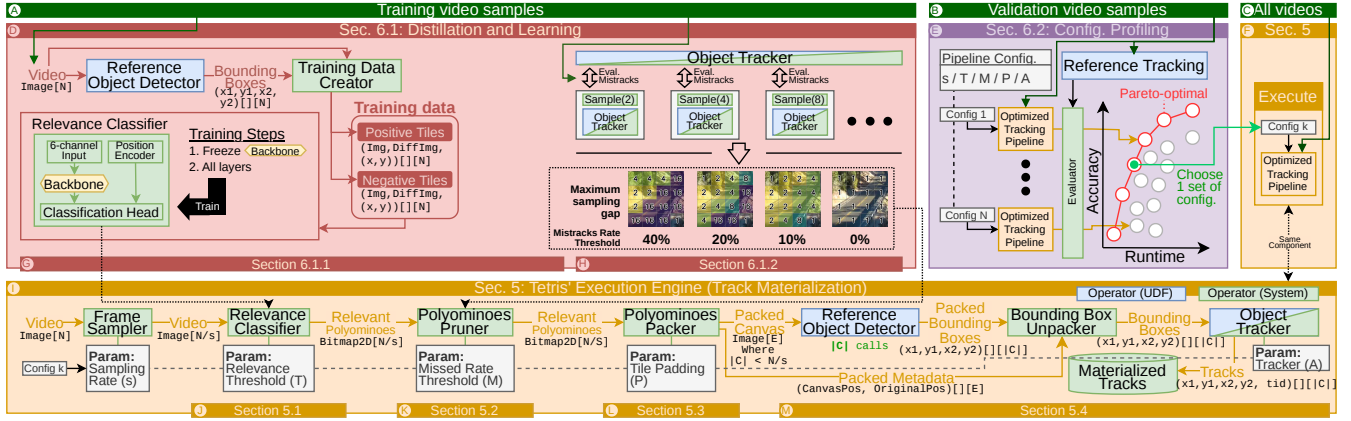
Figure 3: System overview. The learning and Pareto frontier generation stages produce intermediate artifacts: the relevance classifier (§6.1), maximum tile sampling gaps (§6.2), and a throughput-accuracy curve from swept system configurations (§6.3). The user selects a configuration, then the Tetris execution engine (§5) uses it to extract tracks on the full dataset.
