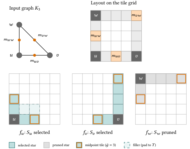
Figure 12: The pruning reduction on the triangle K_3 ( n = 3 , minimum vertex cover size two). Top Left The input graph with each edge’s midpoint marked. Top Right Its layout on the shared tile grid. Midpoint tiles receive gap n = 3 , so their single full-range window forces one endpoint star each; all other tiles carry no sampling gap. Bottom The three frames, one star per vertex, each star padded to T = 7 tiles. Each midpoint is covered by exactly its edge’s two endpoint stars, e.g., m_{vw} by S_v and S_w only, so a feasible selection must pick an endpoint star per edge, i.e., a vertex cover. Selecting S_u and S_v (the cover \{u, v\} ) satisfies all three midpoints at 2T = 14 tiles, and S_w is pruned; no single star covers all three midpoints, matching K_3 ’s cover size of two.
