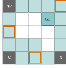
f_0 : U always selected
