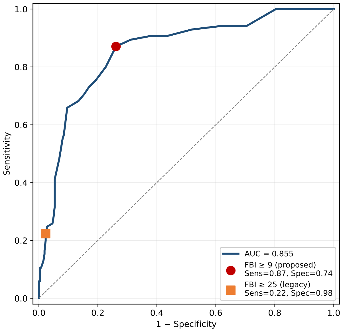
FBI total vs Consensus reference standard (n = 345)
