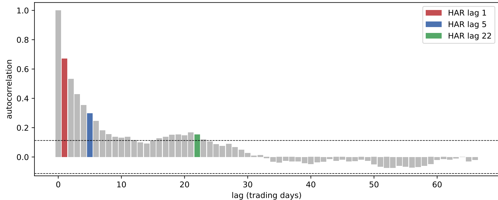
Mean ACF of log-RV (RK) — justifies HAR daily/weekly/monthly
