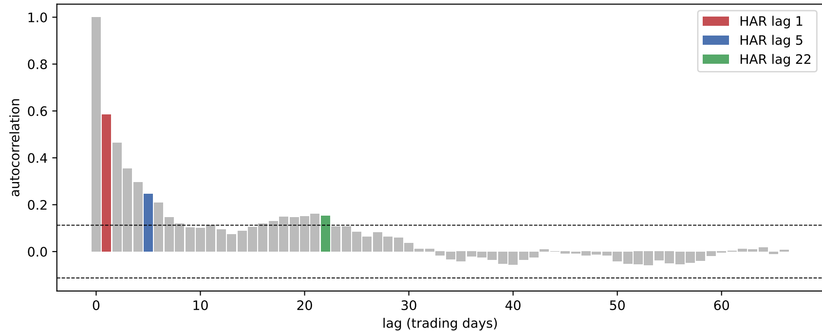
Mean ACF of log-RV (RV) — justifies HAR daily/weekly/monthly
