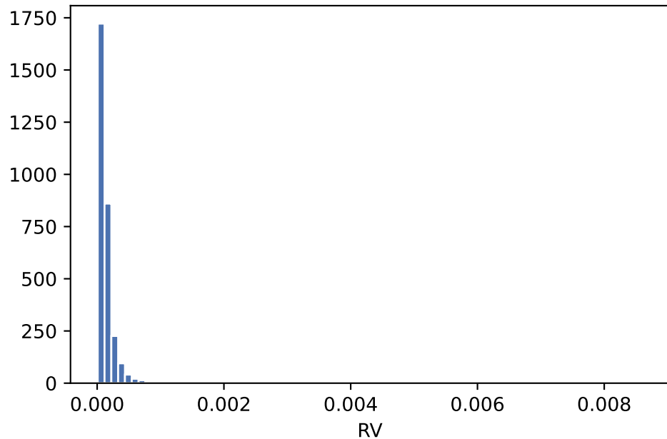
Realized variance (levels, RV)
