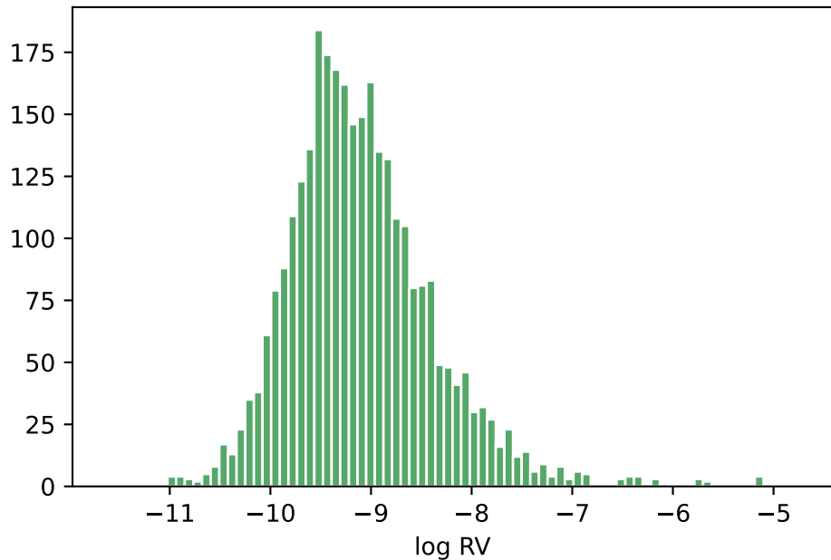
log realized variance (RV)
