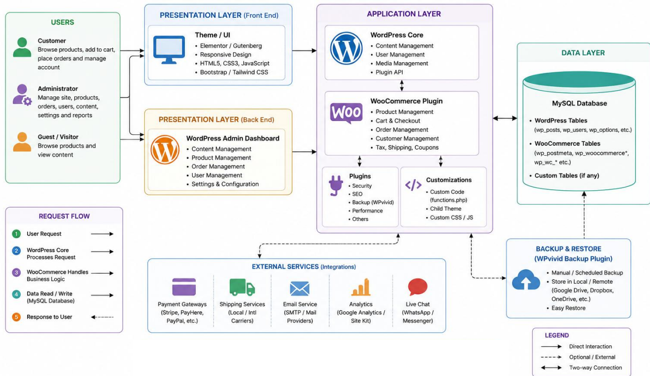
Figure 1. Architecture derived from the WordPress backup, installed theme/plugins and database package information.
