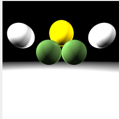
With shader
