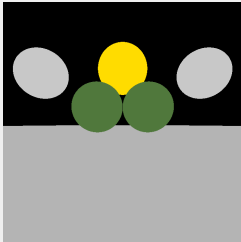
Without shader
