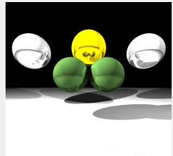
Full
