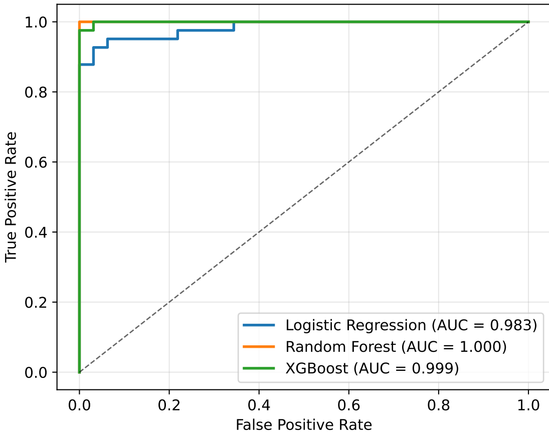
RQ1: ROC Curves — Wildfire Risk Classifiers
