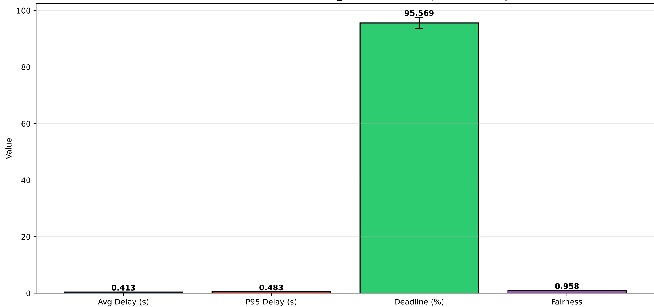
Game-Theoretic Offloading Performance (Mean \pm Std)
