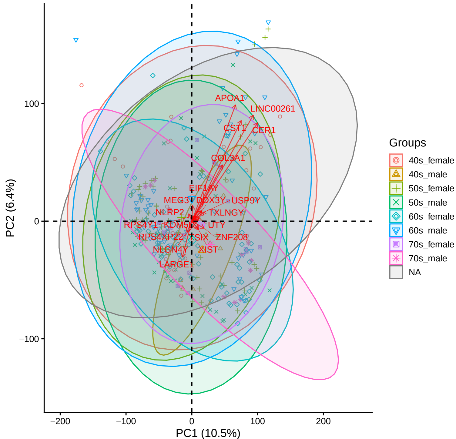
PCA of RNA-seq log 2 (CPM) Data by Age and Sex
